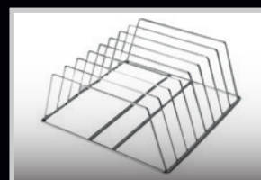
MH103454B: Capacity 8 x 1/1 gastronorm containers – maximum depth 40mm
